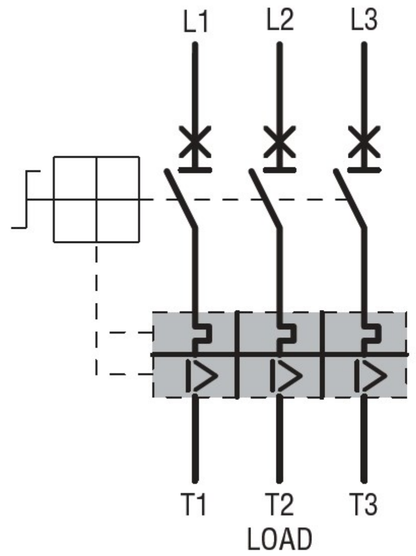
Three-phase LINE
