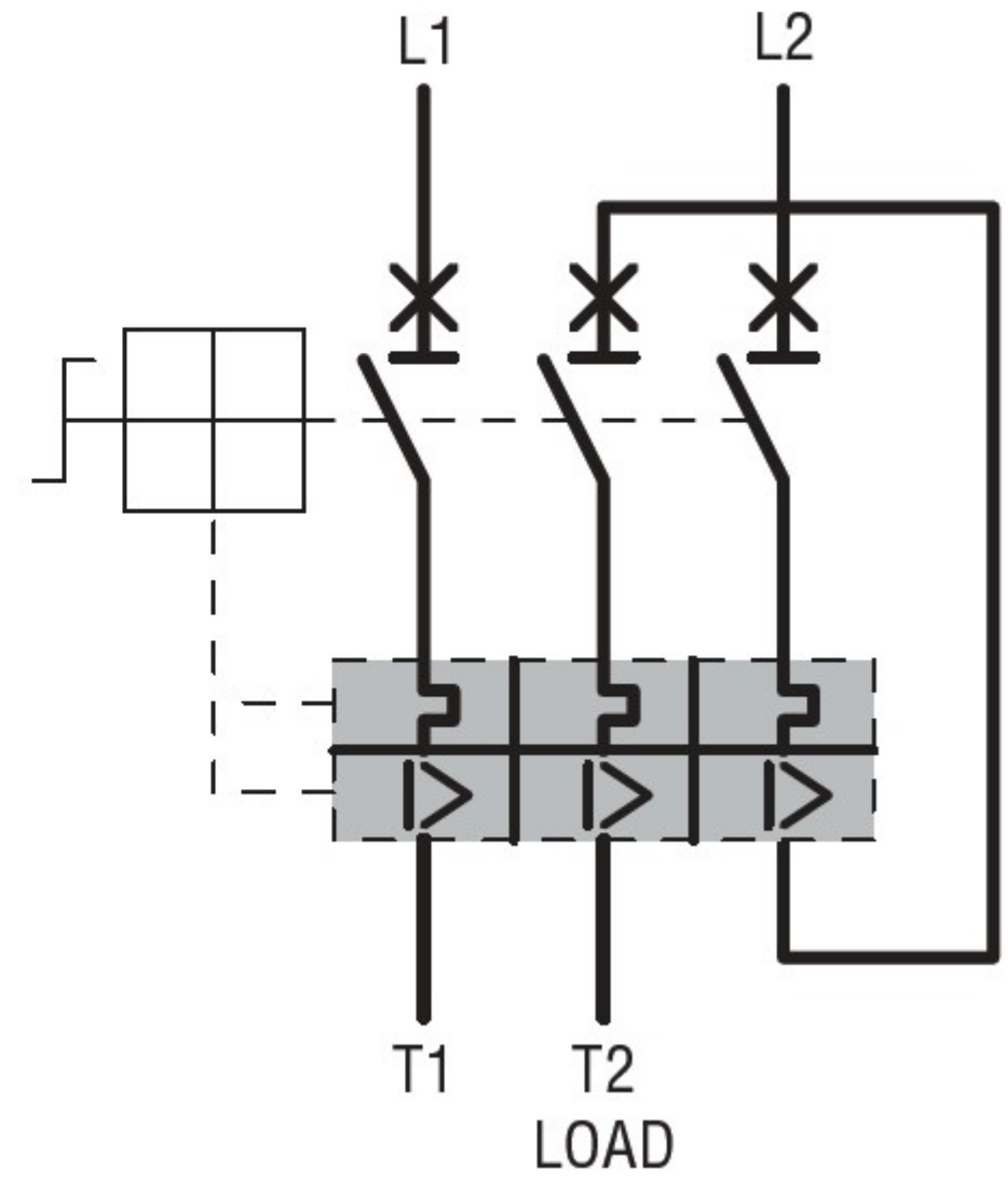
Single-phase and DC LINE
