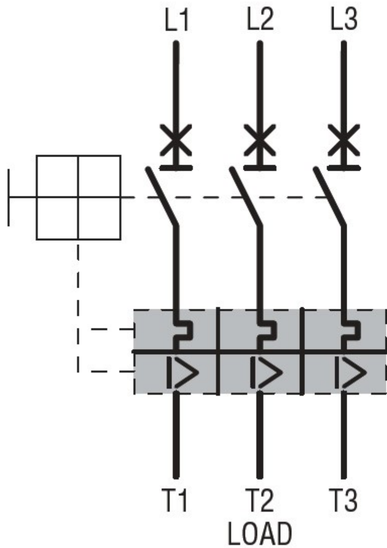
Three-phase LINE
