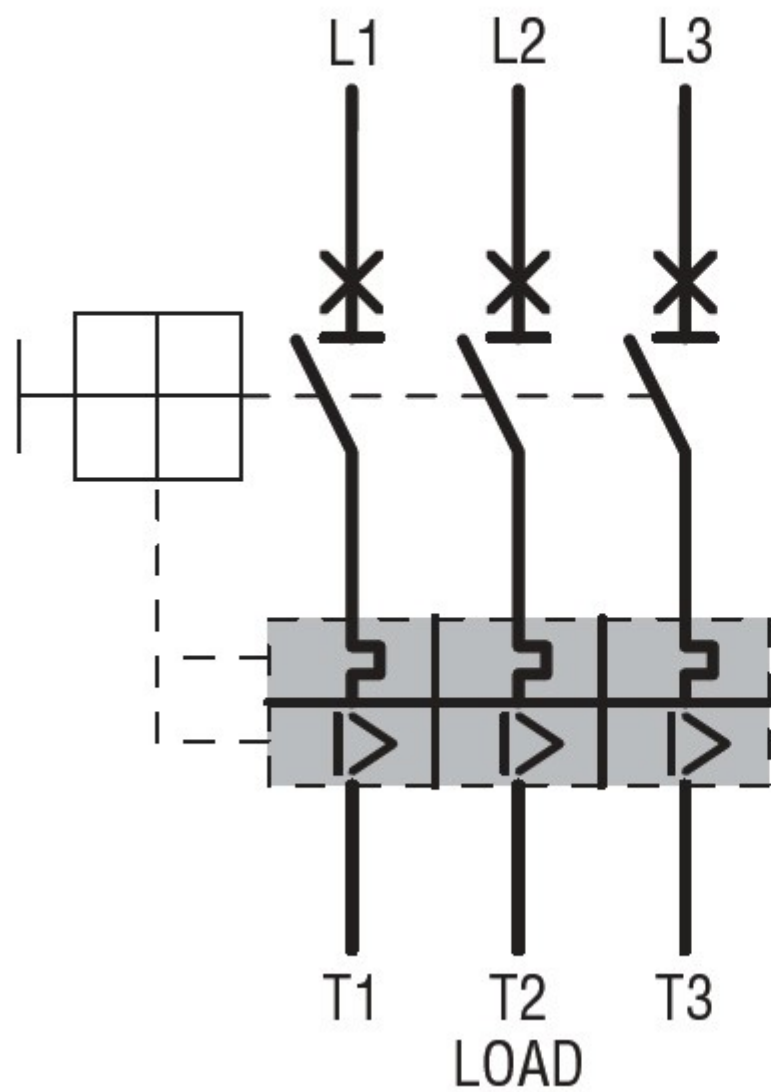
Three-phase LINE
