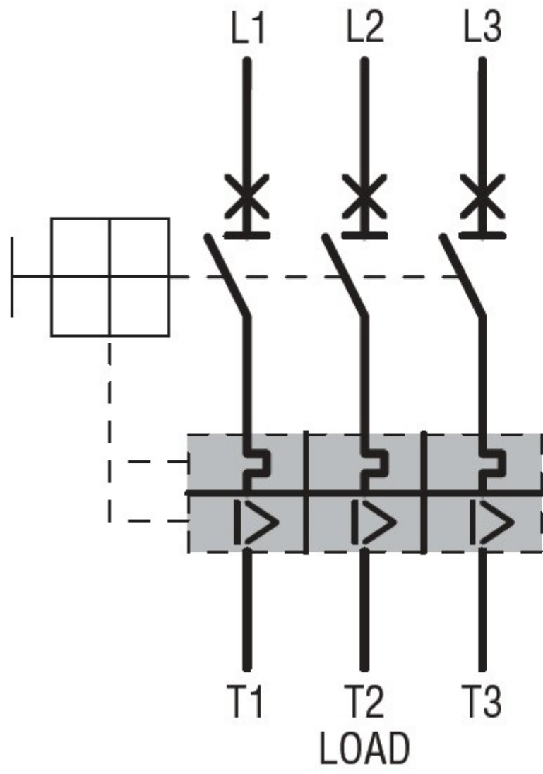
Three-phase LINE
